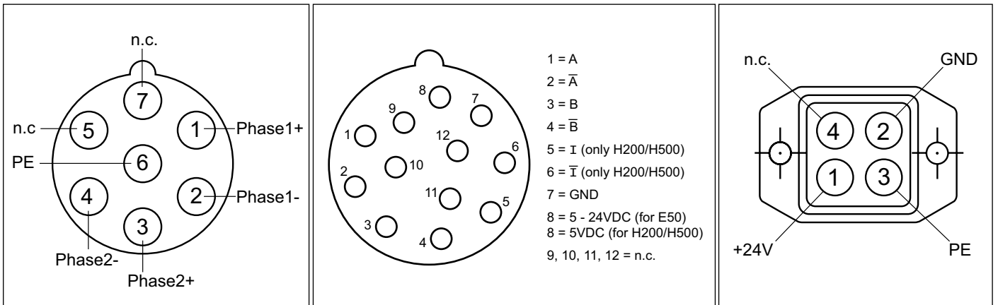
connector motor phases
