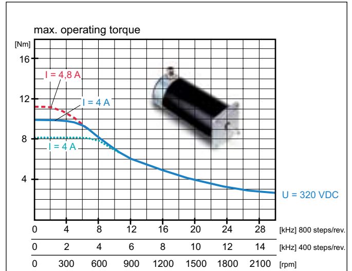
SM 88.4.18M4 with WSE 04.230AC
